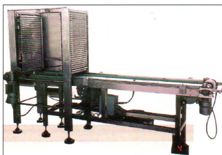
可配置上層自動盤子供給系統 Equipped with over head auto. tray supply system
