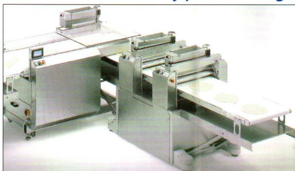
可轉向一次整盤排列 One time whole pan arrangement can be change the direction
